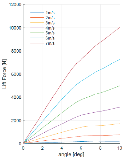
Figure 3: Lift forces for Eppler E 838 profile
