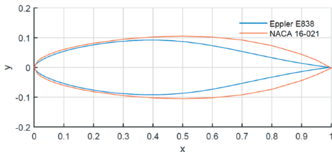
Figure 2: Geometry of NACA 16-021 and Eppler E 838 profiles
